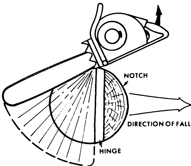
Figure 5-7. Normal felling cut.
